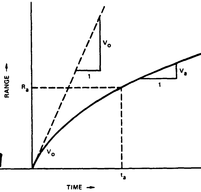
FIGURE 3-22 [REDACTED] TRANSITION FROM INITIAL TO ACOUSTIC-WAVE VELOCITY
